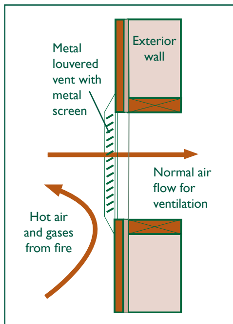
Attic Vent
